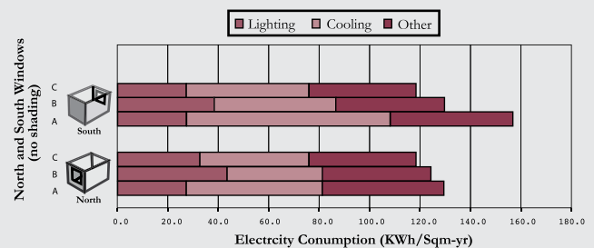
Annual Electricity and cooling Energy use Comparison by Orientation with no shading Window A: single glazing, clear, U=1.25, SHGC = 0.72, VT = 0.7 Window B: double glazing, reflective coating, U=0.54, SHGC = 0.17, VT = 0.1 Window C: double glazing, spec. Selective low-E tint, U=0.46, SHGC = 0.27, VT = 0
