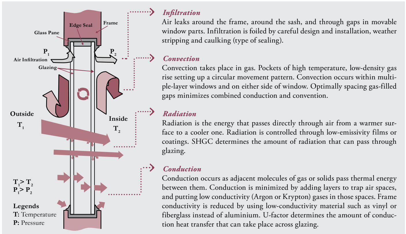
Fig. 8: Heat and Air Movement through Double Glazing Window System Source: Adapted from E Source Technology Atlas
