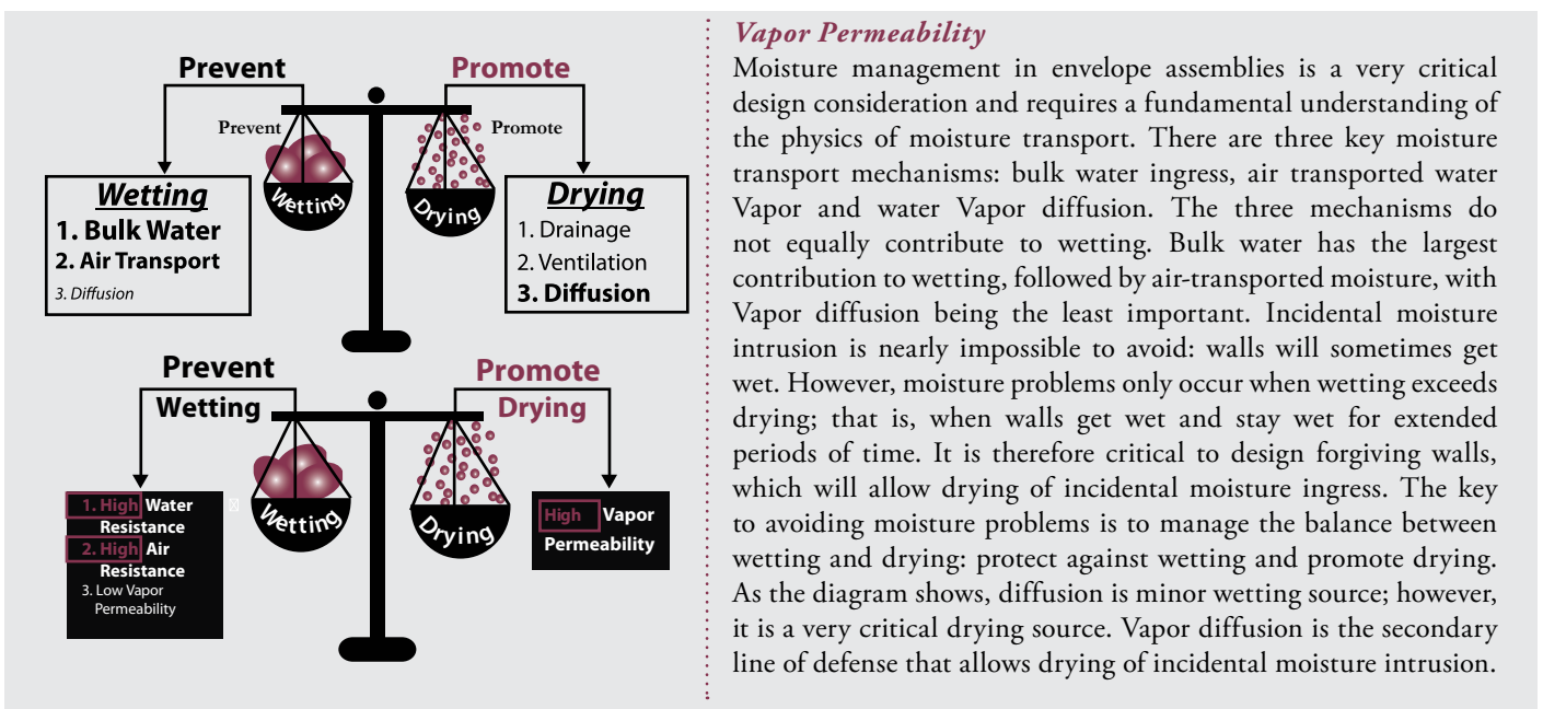
Fig. 4: Moisture/Vapor Management Principles Source: DuPont
