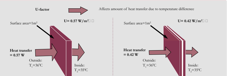
Fig. 3: Illustration of concept of U-factor
