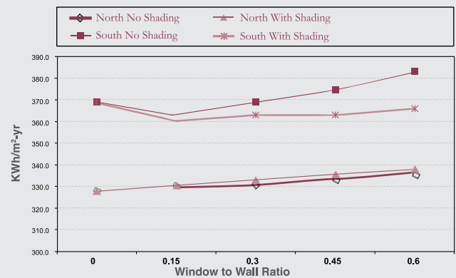
Fig. 6: Impact of Orientation and Shading on Annual Electricity Consumption
