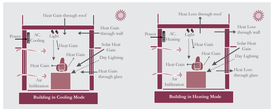
Fig. 1: External and Internal Heat loads
