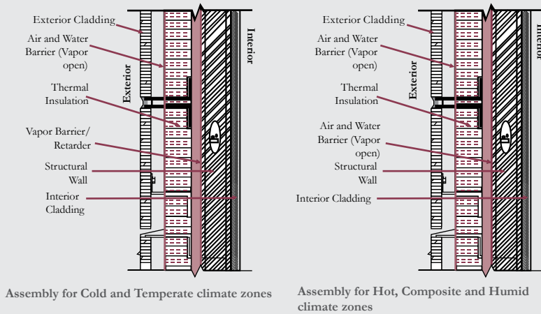
Fig. 7: Schematic Showing the Correct Placement of Barriers. Source: DuPont
