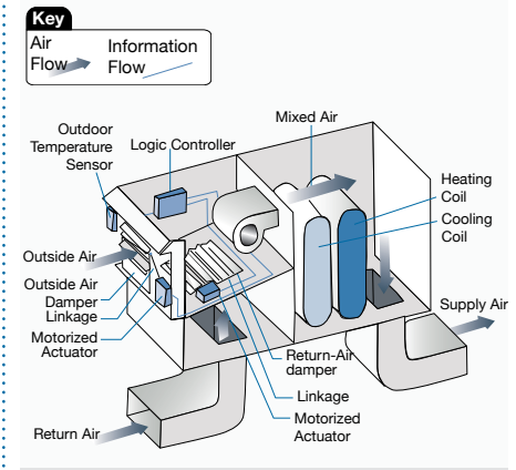
Fig. 4: The Components of an Economizer (Source: E Source Cooling Atlas)
