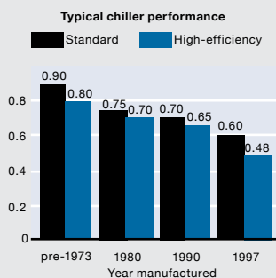
Fig. 8: Trend in Chillers Efficiency (Source: E Source Cooling Atlas)
