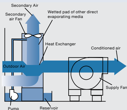
Fig. 5: Indirect Evaporative Cooler (Source: E Source Cooling Atlas)
