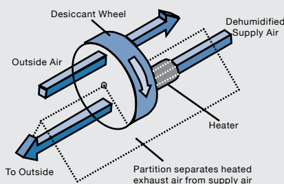
Fig. 6: Solid Desiccant Wheels (Source: E Source Cooling Atlas)
