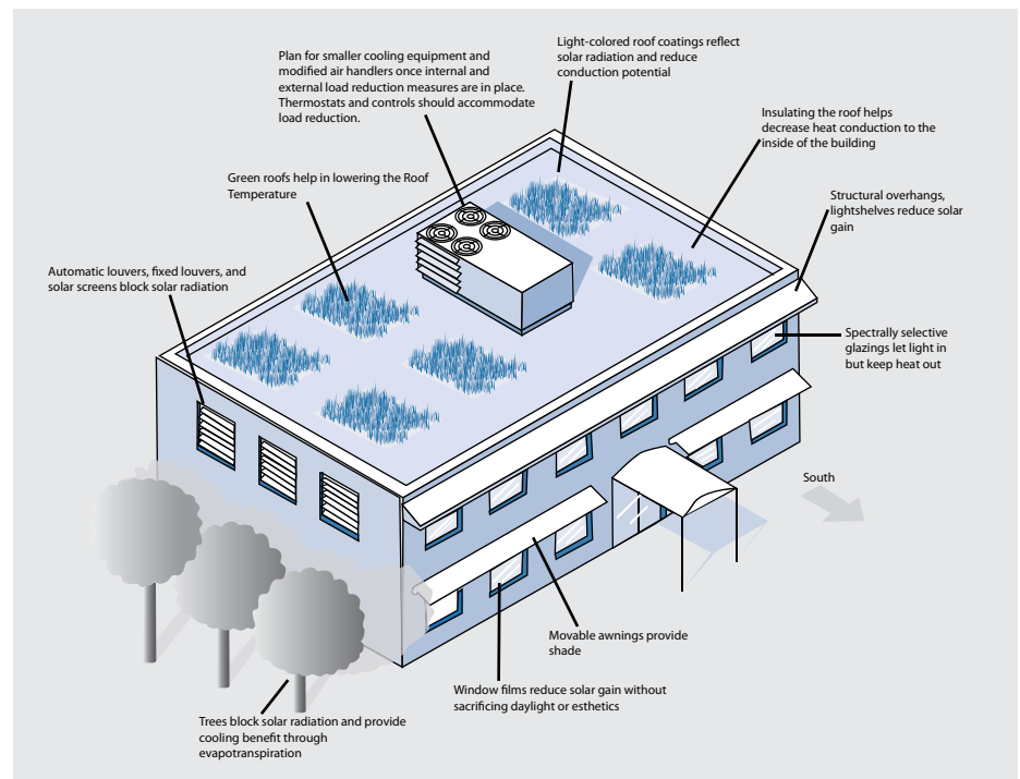
Fig. 1: Cooling Load Reduction Measures (Source: E Source Cooling Atlas)
