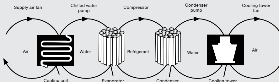
Fig. 7: Process Diagram of a Chilled Water Air-Conditioning (Source: E Source Cooling Atlas)
